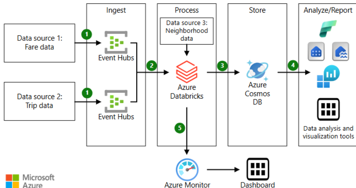
Fig 3: Stream Processing with Databricks
